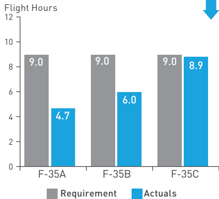
Maintainability: Maintenance Man Hour Per Flight Hour
