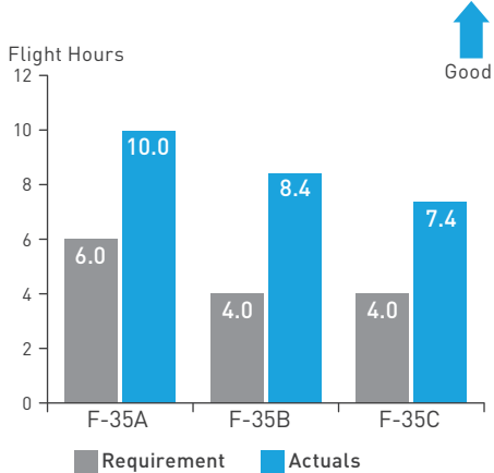
Reliability: Mean Flight Hour Between Failure
