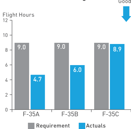
Maintainability: Maintenance Man Hour Per Flight Hour
