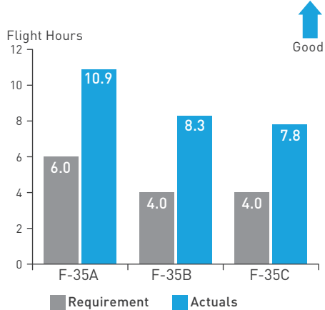
Reliability: Mean Flight Hour Between Failure
