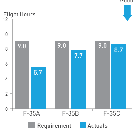
Maintainability: Maintenance Man Hour Per Flight Hour
